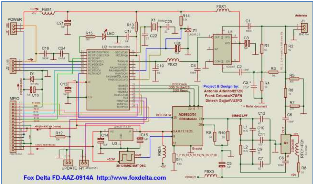
The circuit diagram (FD-AAZ-0914A) of the SWR-Analyzer
