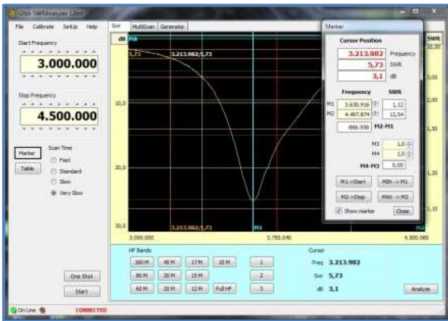
Figure showing Return Loss of 80m band pass filter.
